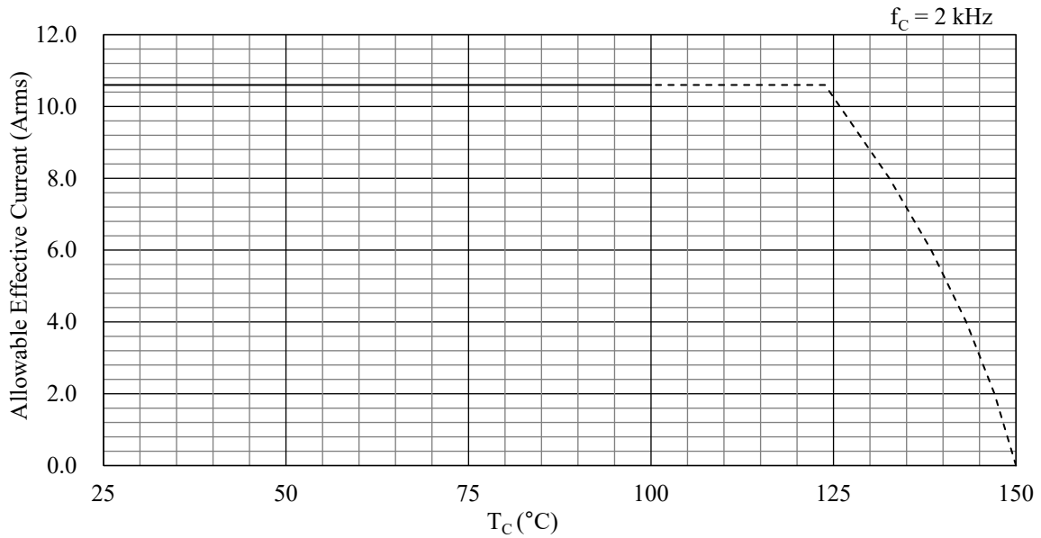
Figure 15-25. Allowable Effective Current ( f_C = 2\text{ kHz} )
