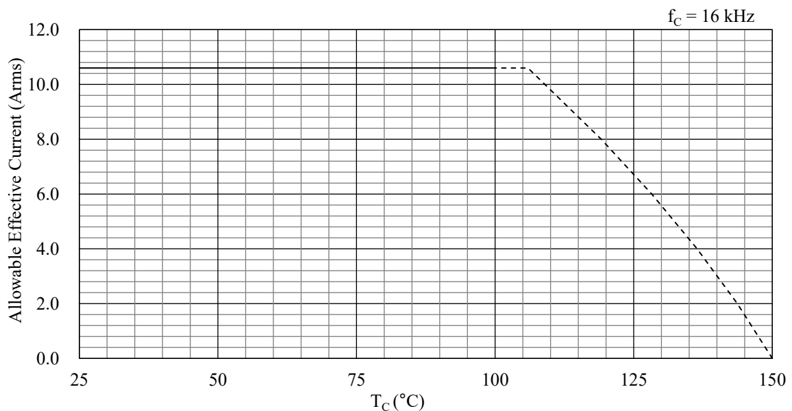
Figure 15-26. Allowable Effective Current ( f_C = 16\text{ kHz} )
